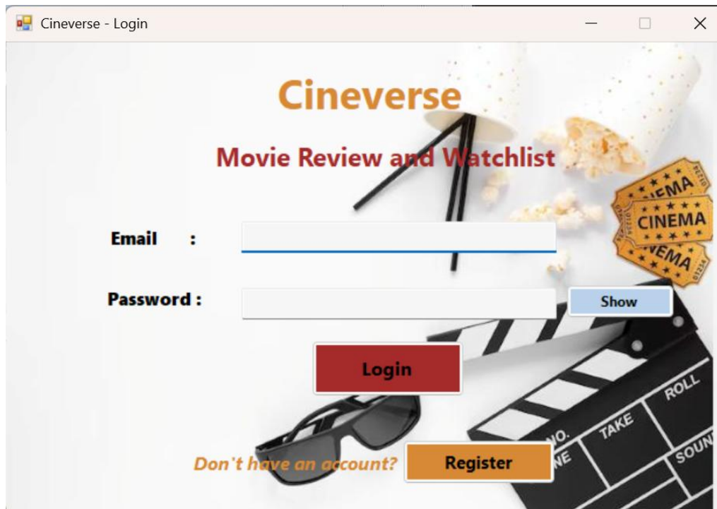
Fig 5.1: Login Screen
