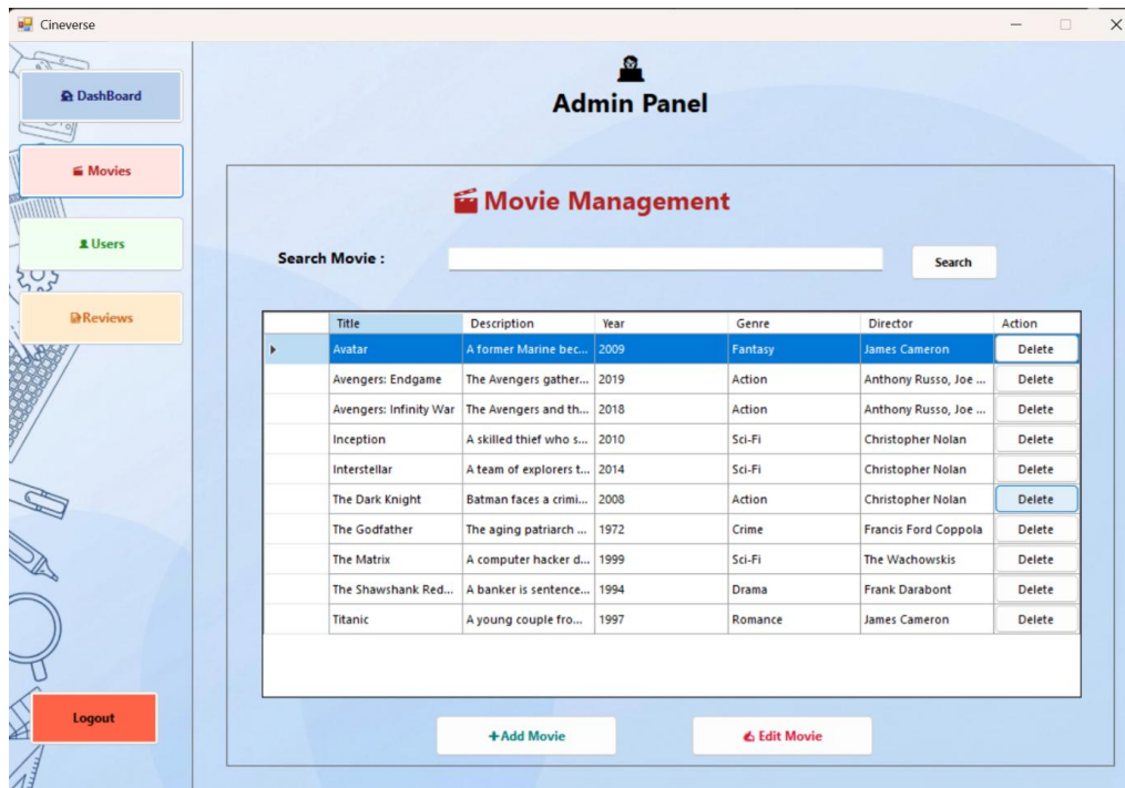
Fig 5.10: Movie Management
