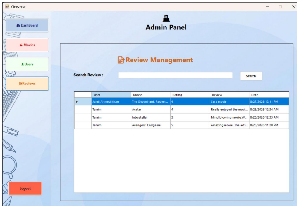
Fig 5.14: Review Management
